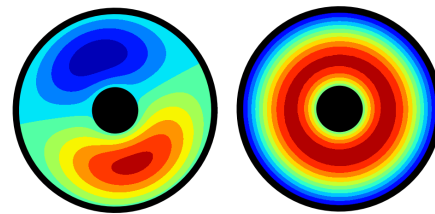
FIG. 6 – "Mixed" (left) and "continuous" (right) minimal-ensrophy solutions obtained.
