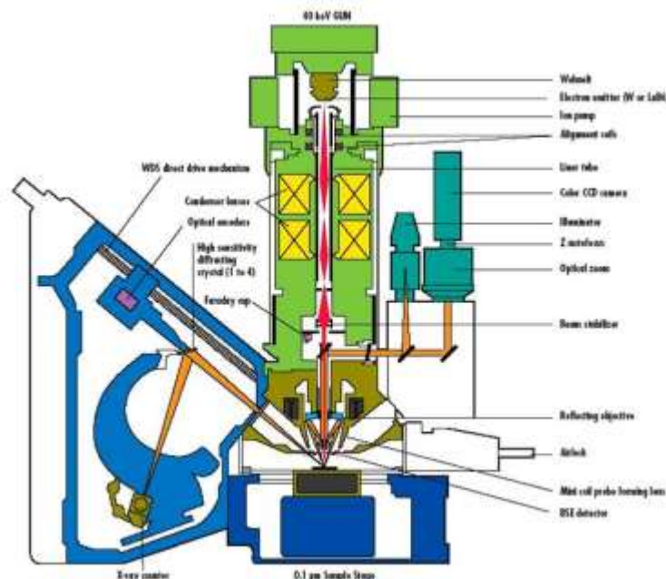
Figure 6 : Diagram of an EPMA device [13].
